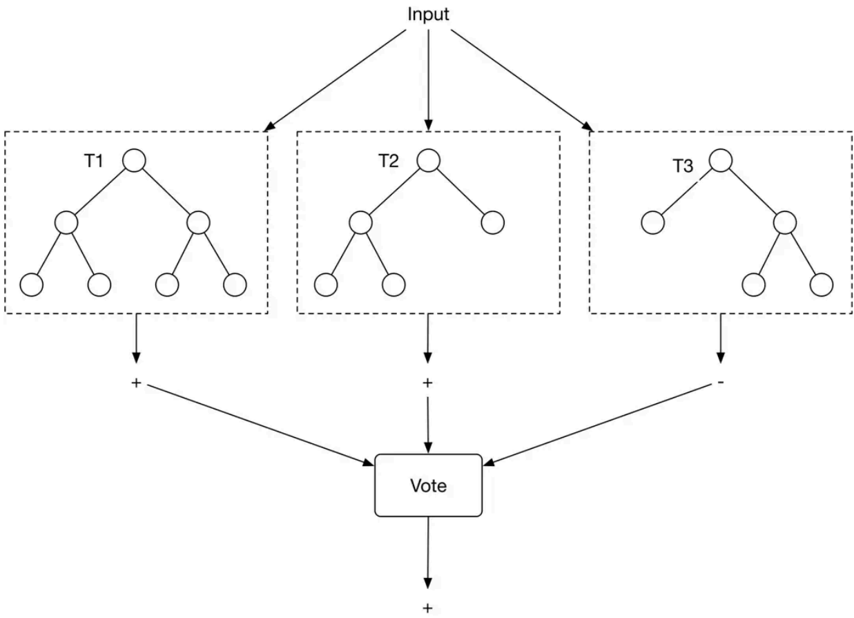
Figure 7.14: Random forest
